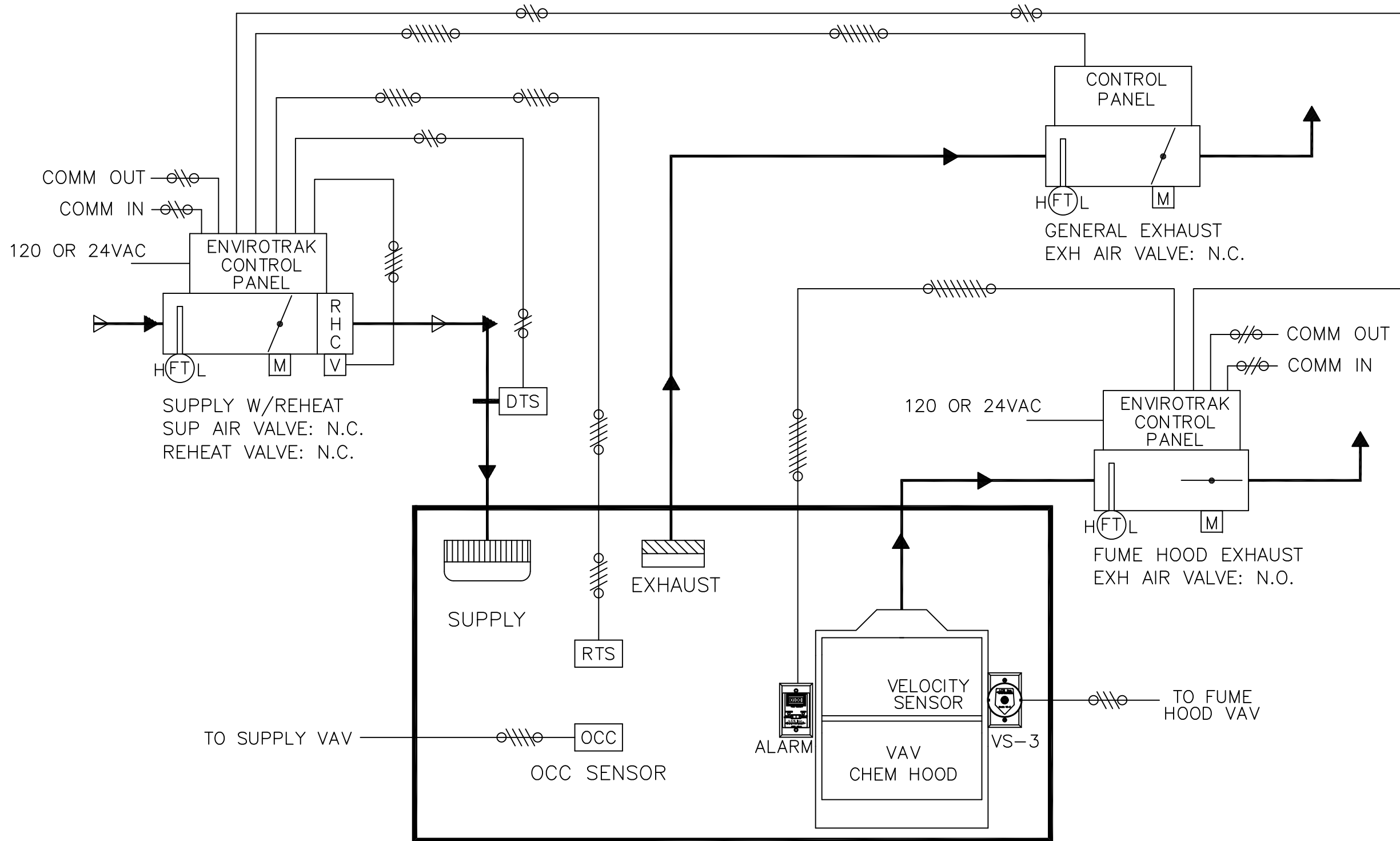
AIRFLOW AND FIELD WIRING DIAGRAM FUME HOOD FACE VELOCITY CONTROL WITH AIRFLOW TRACKING AND OCCUPANCY SENSING
