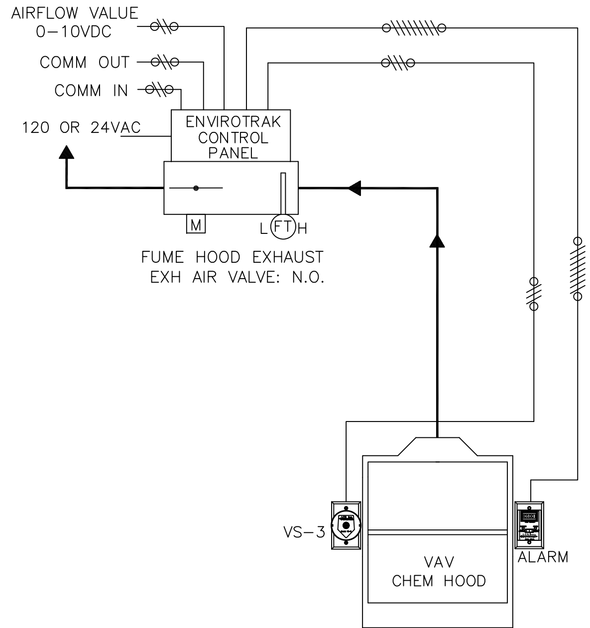
AIRFLOW AND FIELD WIRING DIAGRAM STAND-ALONE FUME HOOD FACE VELOCITY CONTROL
