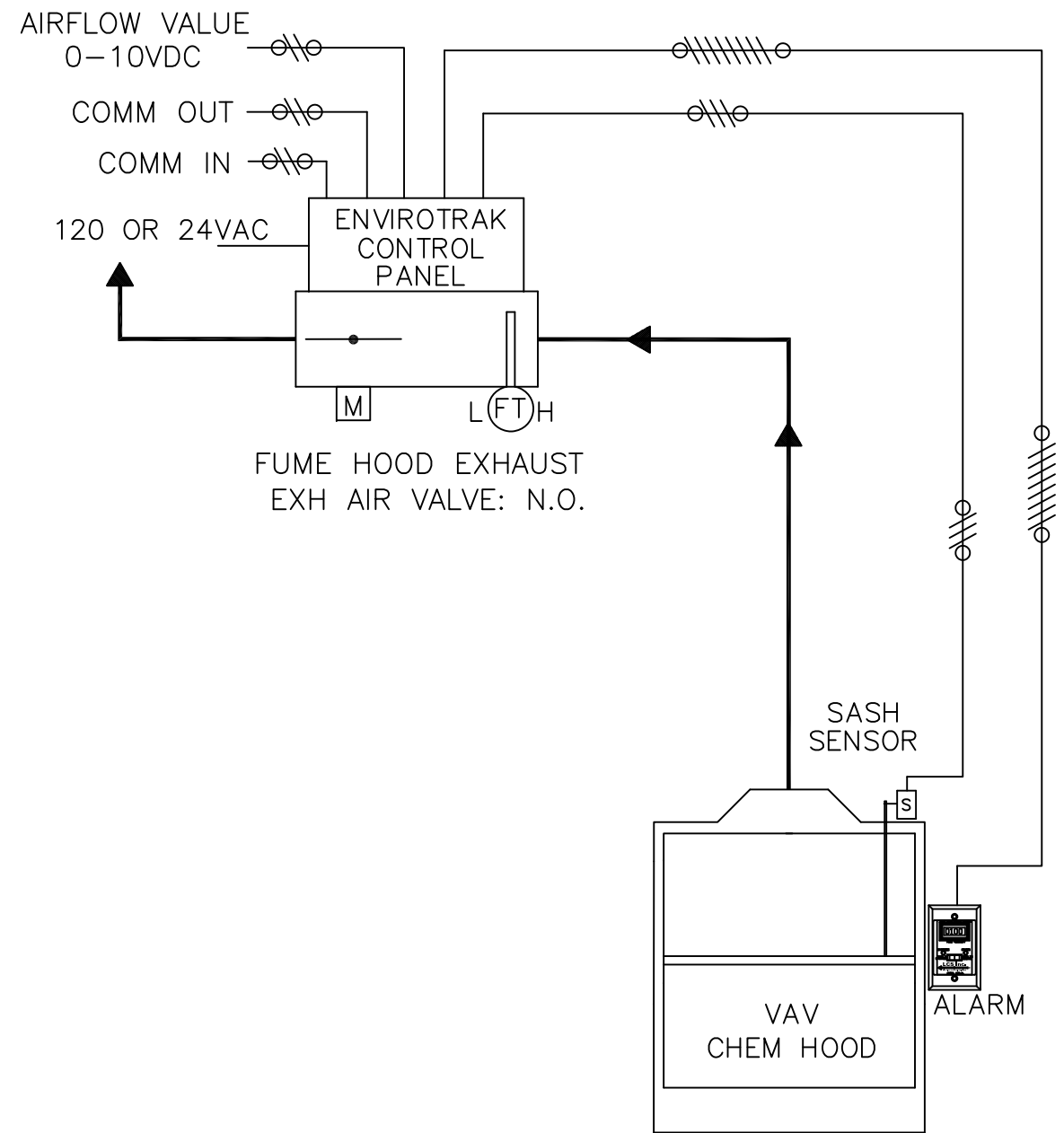
AIRFLOW AND FIELD WIRING DIAGRAM STAND-ALONE FUME HOOD SASH POSITION CONTROL
